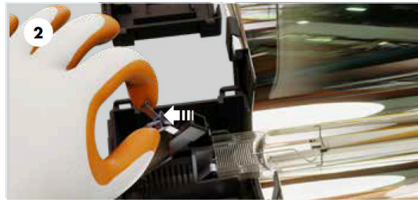
2 Slide both fittings fully open, as shown
